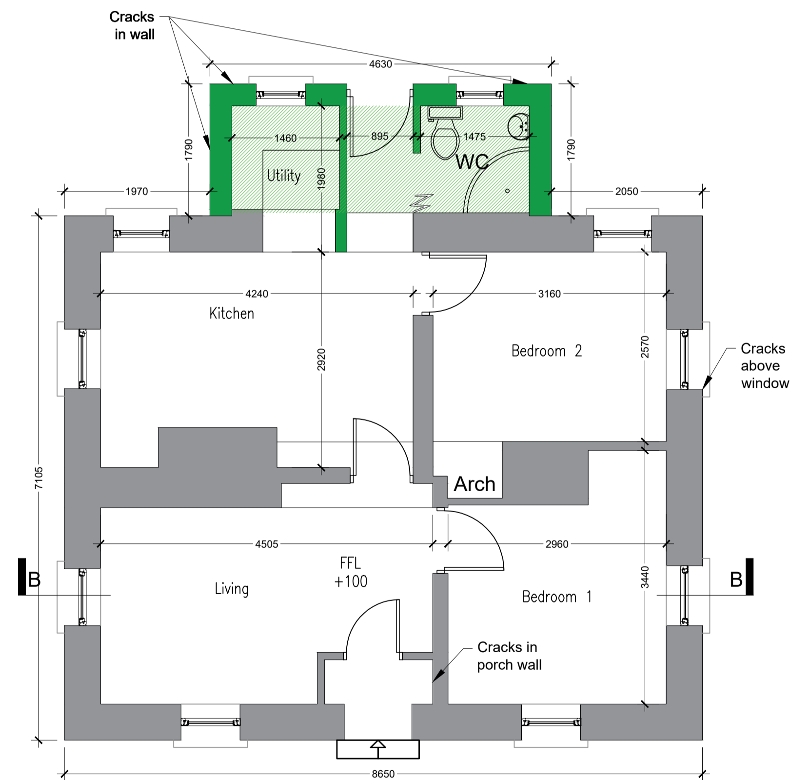
Floor plan scale 1-50
