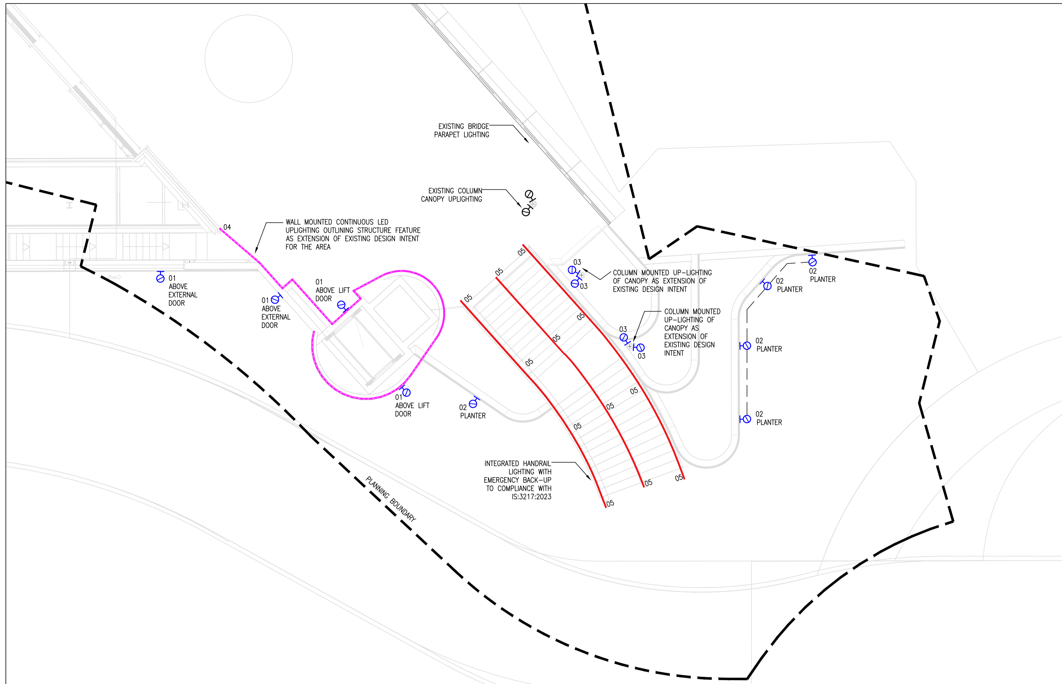
LIGHTING PROPOSAL SCALE 1:100
